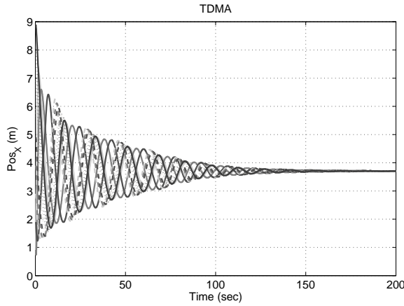
Fig. 10: Multi-agent consensus using TDMA
