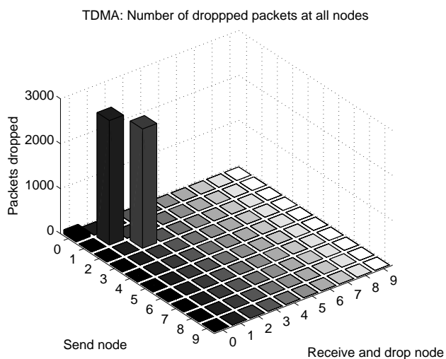
Fig. 3: Packet drop using TDMA. Simulation time = 60 sec.
