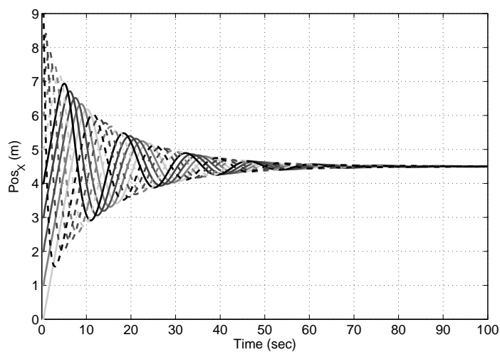
Fig. 6: Multiple quadrotor consensus with \tau_{ji} = \tau_{kj}
