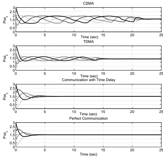
Fig. 11: Comparison of convergence time for different MAC algorithms
