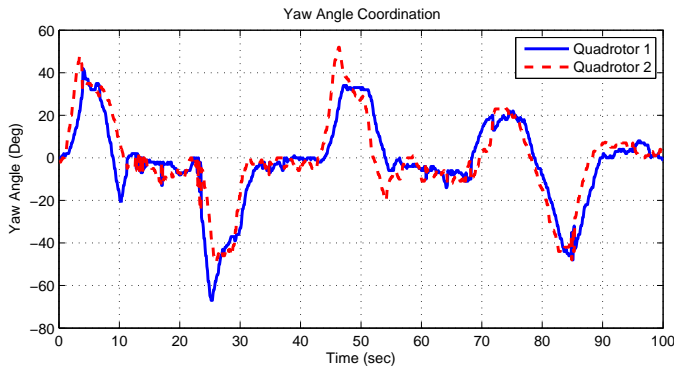
Fig. 12: Average consensus for the yaw subsystem. An external reference was given to the system in order to show the delay over the wireless network
