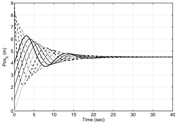
Fig. 2: Multiple quadrotor consensus using perfect communication
