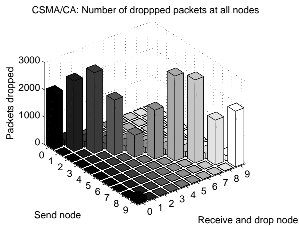
Fig. 4: Packet drop using CSMA/CA. Simulation time = 60 sec.
