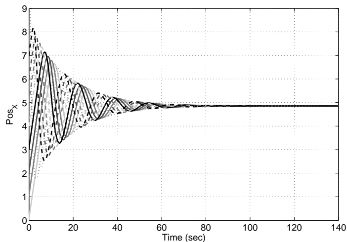
Fig. 7: Multiple quadrotor with \tau_{ji} \neq \tau_{kj}
