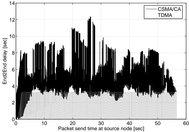
Fig. 5: End-2-End delay comparison between CSMA/CA and TDMA. Simulation time = 60 sec.
