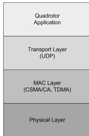
Fig. 8: Multiple quadrotor wireless network stack
