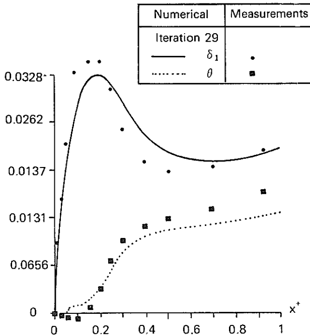
Fig. 3. — Comparison of the numerical results and measurements for \delta_1 and \theta .
