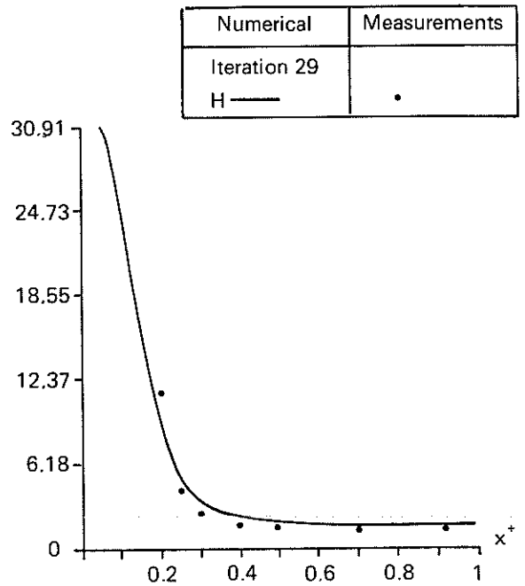
Fig. 4. — Comparison of the numerical results and measurements for H .
