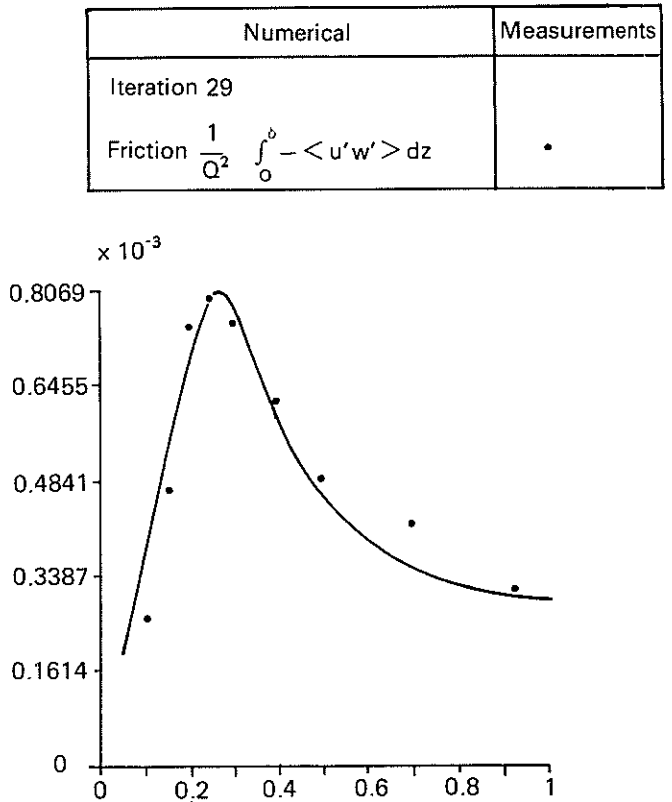
Fig. 5. — Comparison of the numerical results and measurements for integral turbulent friction.
