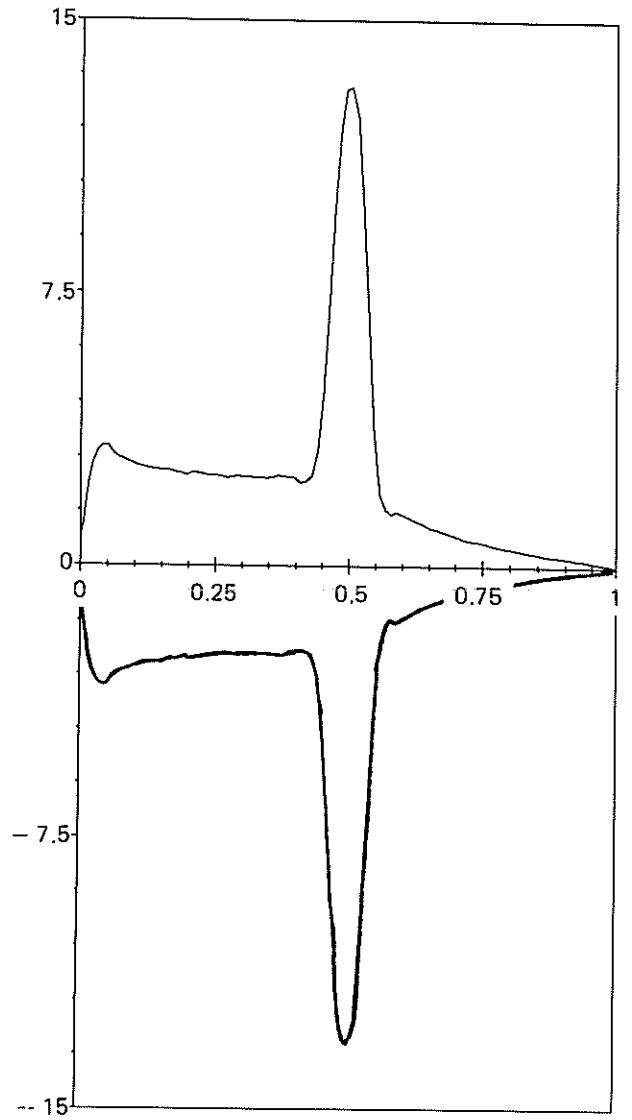
Fig. 34. — Harmonic 1, real part. NACA12 airfoil, Mach 0.80, steady angle of attack 0 degrees. Movement: forward quarter pitch, amplitude 1 degree, reduced frequency K=0.25 . Unsteady pressure coefficient. — Lower surface, - - - Upper surface.
