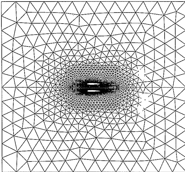
Fig. 11. — Complete view of the mesh of the computation domain. Biplane NACA12 airfoil.
