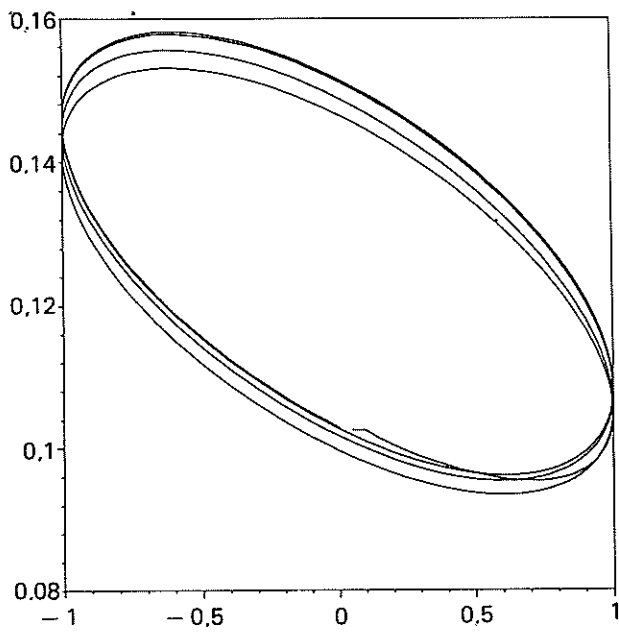
Fig. 26. — Lissajous figure for forward quarter moment. Movement: forward quarter pitch, amplitude 1 degree, reduced frequency K=2 .
