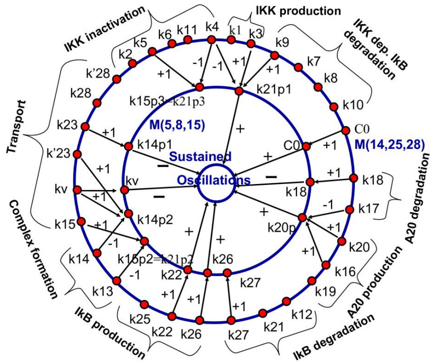
Figure 7: The model \mathcal{M}(14, 25, 28) from [76] (first proposed in [61]) was used to generate a hierarchy of simpler models, the simplest one being \mathcal{M}(5, 8, 15) . We show the mapping between the parameters of the models \mathcal{M}(14, 25, 28) and \mathcal{M}(5, 8, 15) . Parameters of the first model are gathered into monomials that are parameters of the reduced model. The integers on the arrows connecting parameters represent the corresponding powers of the parameters in the monomial. The innermost circle represents a dynamical property of the model that is influenced positively, negatively, or negligibly by the effective parameters (parameters of the reduced model). From [79].
