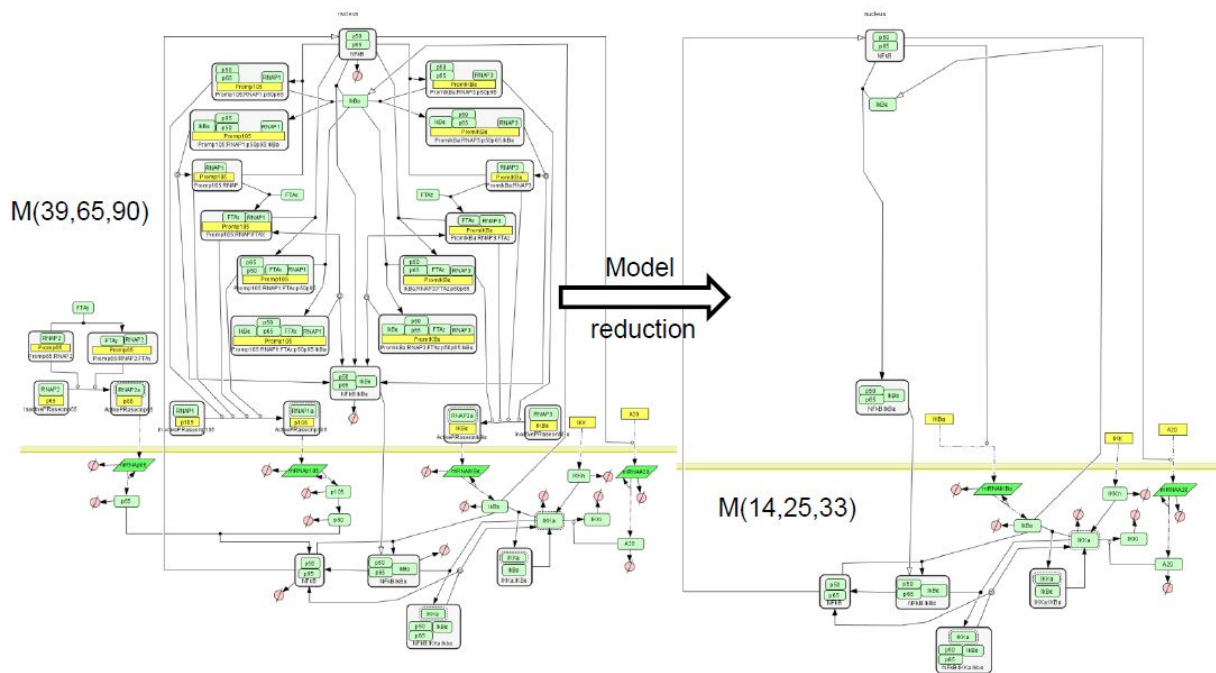
Figure 6: Model of NF- \kappa B signaling, proposing separate production of the subunits p50, p65, the full combinatorics of their interactions as well as with the inhibitor I \kappa B, the positive self-regulation of p50, and in addition an A20 molecule whose production is enhanced upon NF- \kappa B stimulation, and which negatively regulates the activity of the stimulus responding kinase IKK [76]. This model, denoted \mathcal{M}(39, 65, 90) contains 39 species, 65 reactions and 90 parameters. We have reduced it to various levels of complexity. Among the reduced model we obtained one, \mathcal{M}(14, 25, 33) that has the same stoichiometry as a model published elsewhere by another author [61] and denoted \mathcal{M}(14, 25, 28) . Incidentally, this is also the simplest model in the hierarchy related to \mathcal{M}(39, 65, 90) . The rate functions in the reduced model are different, explaining the difference in number of parameters. Comparison of the rate functions and of the trajectories of the models \mathcal{M}(14, 25, 33) and \mathcal{M}(14, 25, 28) provided insight into the consequences of various mechanistic modeling choices.
