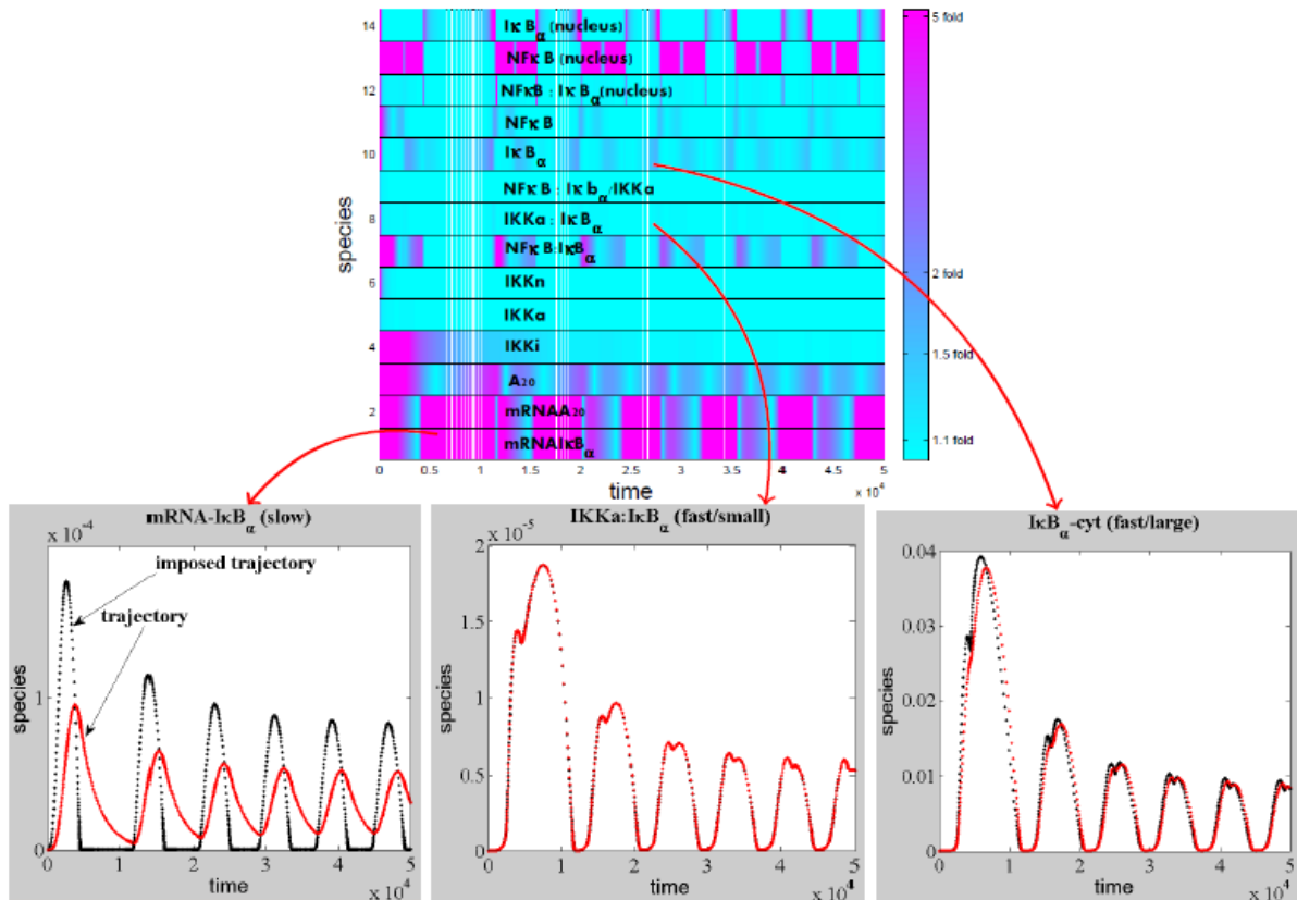
Figure 5: The ratio of the imposed and actual trajectories has been calculated as a function of time for each species of the model of NF\kappa B canonical pathway (proposed in [61], model \mathcal{M}(14, 25, 28) from [76]). If this ratio is close to one fold, the species is slaved, otherwise the species is slow. Among the slaved species, some have low concentrations and satisfy quasi-steady-state conditions, whereas other have large concentrations and satisfy quasi-equilibrium conditions.
