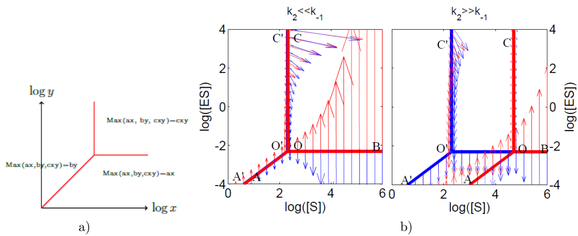
Figure 3: a) The tropical manifold of the polynomial ax + by + cxy on “logarithmic paper” is a three lines tripod. b) The tropical manifolds for the species ES (in red) and S (in blue) for the Michaelis-Menten mechanism. The tropicalized flow is also represented on both sides of the tropical manifolds (with arrows, red on one side, blue on the other side). Sliding modes correspond to blue and red arrows pointing in opposite directions.
