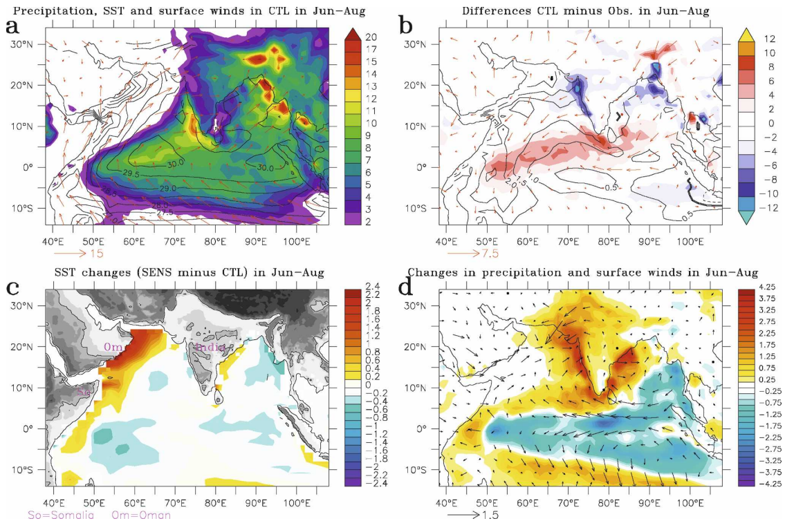
FIG. 2. Summer monsoon in (a) the CTL experiment, (b) differences with observations, and changes in (c) SST and (d) precipitation in the SENS experiment: in (a) precipitation (colors, mm day -1 ), SST (black contours, °C), and 10-m winds (red arrows, m s -1 ) in CTL. (b) Differences with observations (i.e., between Figs. 2a and 1c; note that wind scale has been doubled to better see the biases of the coupled model). Difference SENS - CTL in (c) SST (colors, °C) and (d) precipitation (colors, mm day -1 ) and 10-m winds (arrows). Land topography is added in (c): levels every 250 m between 0 and 1000 m and a black contour at 500 m highlights the Western Ghats (mountains) along the Indian west coast, with altitude between 500 and 1000 m, and other mountain ranges that anchor precipitation (Xie et al. 2006).
