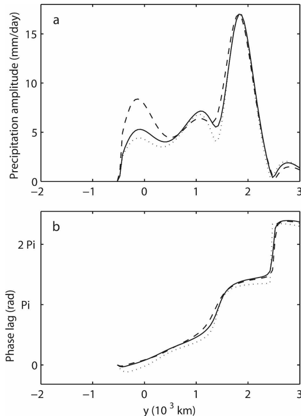
FIG. 4. (a) Amplitude and (b) phase of the precipitation the uncoupled mode (dotted), the coupled mode (solid), and the coupled mode without CRF (dashed).
