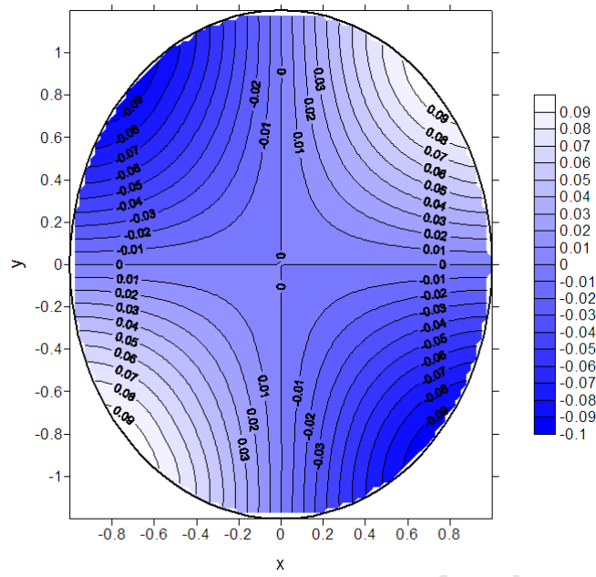
Figure 5: Contours of the warping surface of the elliptical micro-bar
