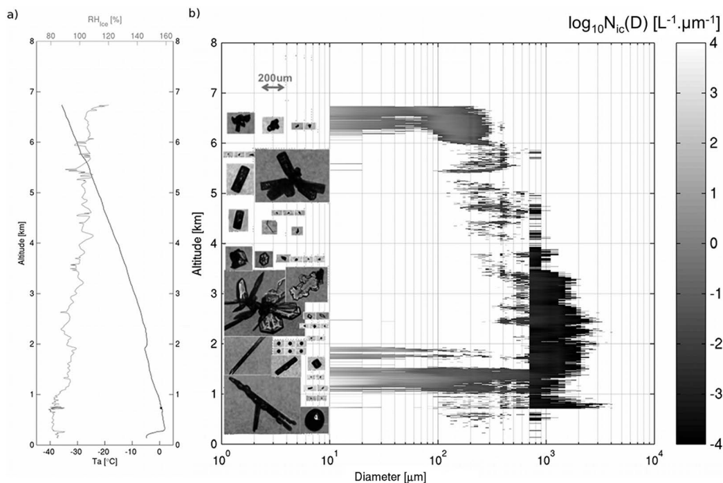
Figure 9. (a) Air temperature from the reverse-flow probe and relative humidity over ice from the EG&G chilled mirror hygrometer. (b) N(D) ( L^{-1} \mu m^{-1} ) as a function of ice crystal diameter ( \mu m ) from 2DS (10–800 \mu m ) and 2DP (>800 \mu m ) observed during F9. CPI images above show representative crystal shape and size to the corresponding altitude for the profile of F9 (1 April 2008) for the time interval 23:13:43–23:45:43 UTC.
