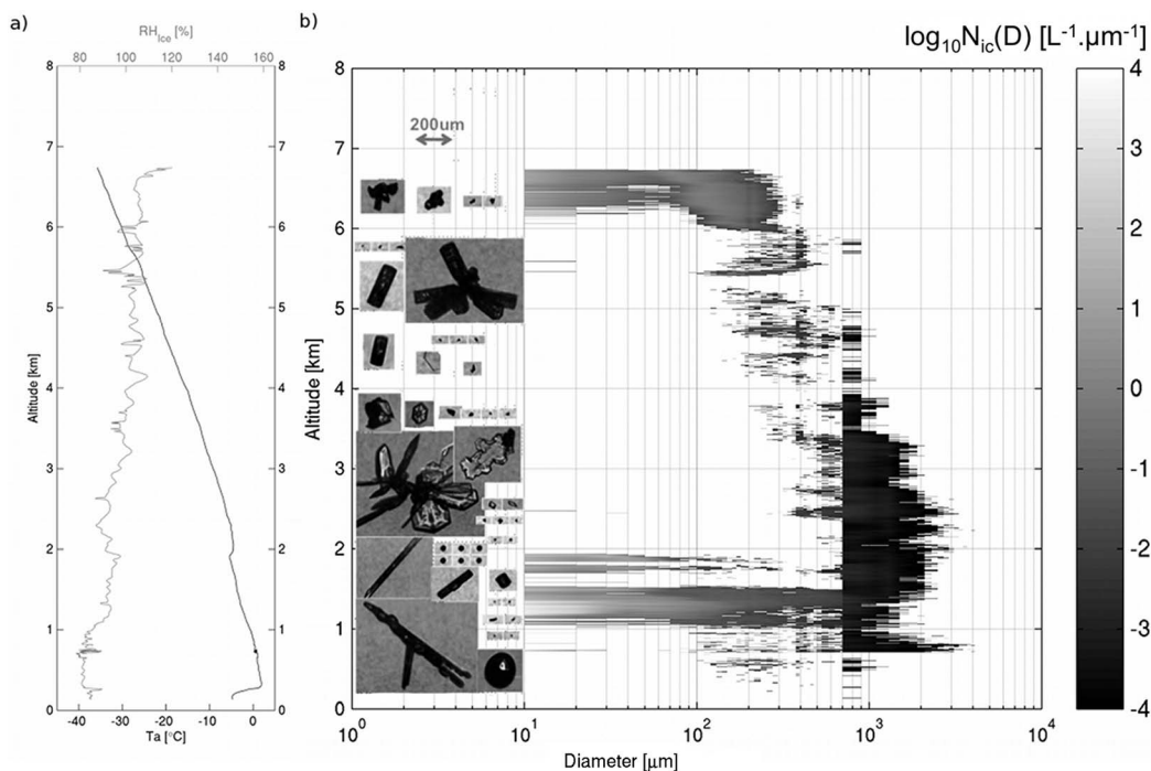
Figure 9. (a) Air temperature from the reverse-flow probe and relative humidity over ice from the EG&G chilled mirror hygrometer. (b) N(D) ( \text{L}^{-1} \mu\text{m}^{-1} ) as a function of ice crystal diameter ( \mu\text{m} ) from 2DS (10–800 \mu\text{m} ) and 2DP (>800 \mu\text{m} ) observed during F9. CPI images above show representative crystal shape and size to the corresponding altitude for the profile of F9 (1 April 2008) for the time interval 23:13:43–23:45:43 UTC.
