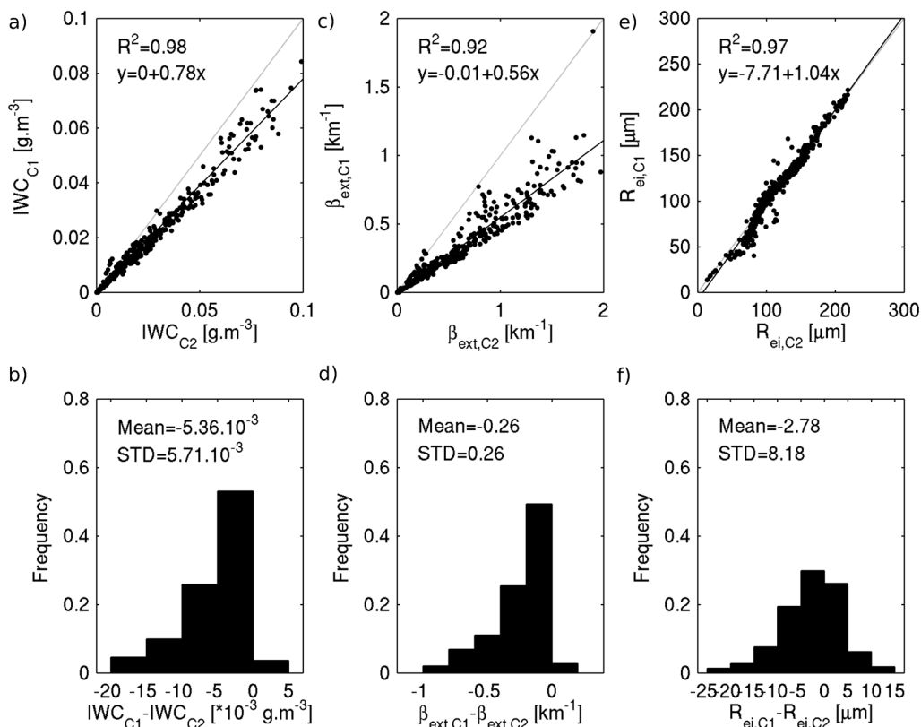
Figure 3. Comparison of (a, b) IWC, (c, d) \beta_{\text{ext}} and (e, f) R_{\text{ri}} from combinations (1) 2DS for N_{[10<D<150\mu\text{m}]} , 2 DC for N_{[150<D<800\mu\text{m}]} , 2DP for N_{[D>800\mu\text{m}]} and (2) 2DS for N_{[10<D<800\mu\text{m}]} , 2DP for N_{[D>800\mu\text{m}]} for ice clouds defined in Table 1.
