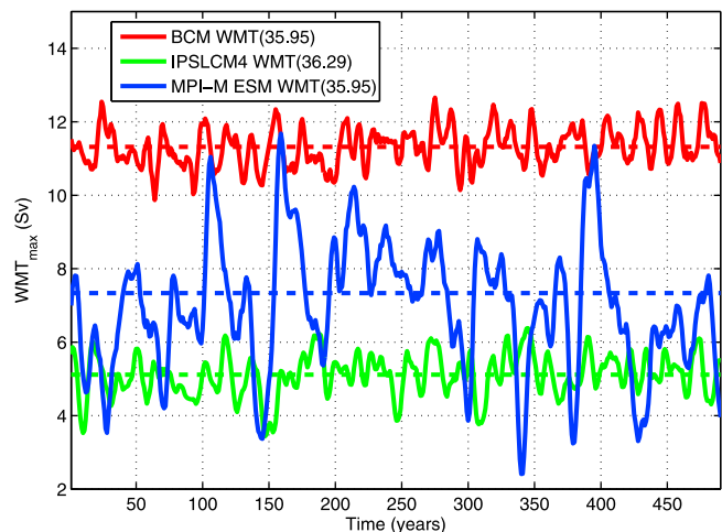
Figure 14. Time series of maximum surface forced water mass transformation in the eastern subpolar region (WMT _{\max} ). The WMT _{\max} and the corresponding \sigma_2 -density (indicated in the legend) for each model were found in Figure 3. The time series are filtered using an 11-year low-pass filter. The dashed lines illustrate the mean WMT _{\max} for each model.
