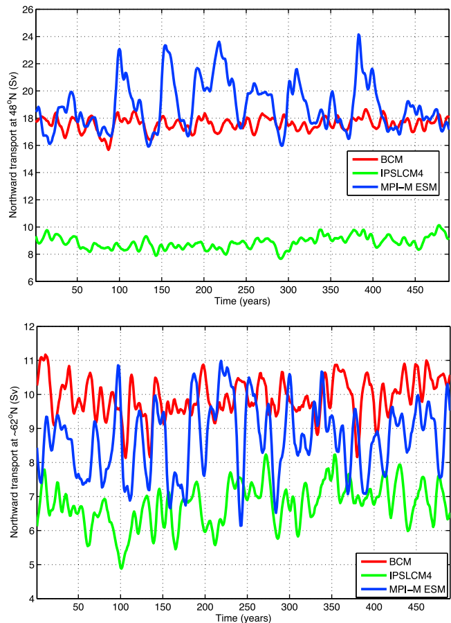
Figure 17. Northward transport at (top) 48^{\circ}\text{N} and (bottom) 60\text{--}64^{\circ}\text{N} . The northward transports are the integrated positive volume transport in density space. The time series are filtered using a 11-year low-pass filter.
