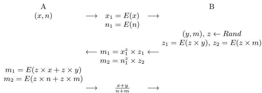
Fig. 1. Privacy preserving Weighted Average Protocol based on Benaloh' scheme E , introduced in [29]
