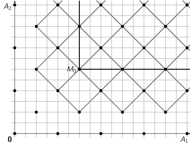
Figure 3: Black dots are the points of the lattice generated by \mathcal{V} . The lattice fundamental regions (formed by the basis) are delimited by the gray lines.
