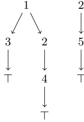
Fig. 2. Representation of set of sets \{\{1, 2, 4\}, \{1, 3\}, \{2, 5\}\}
