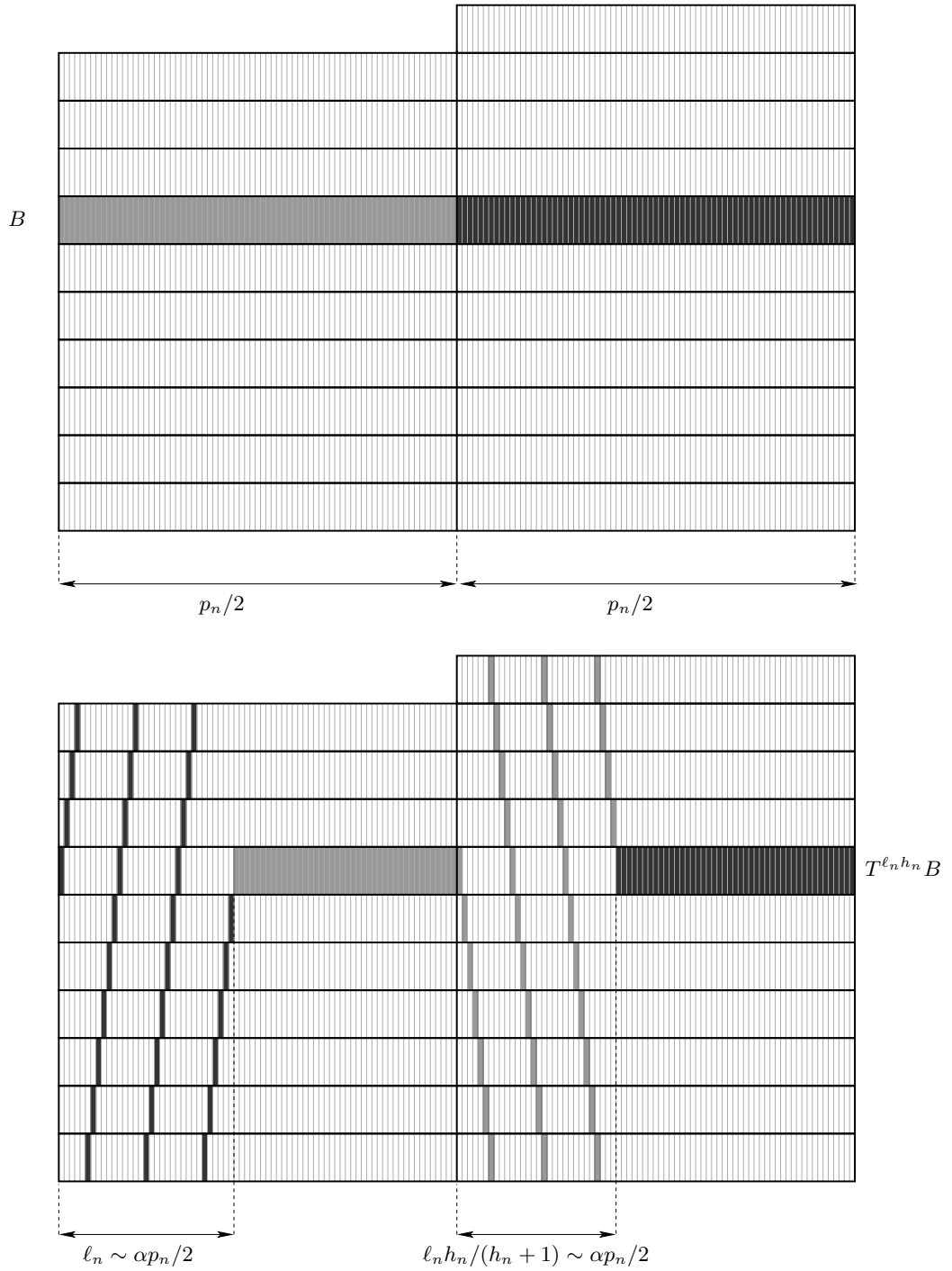
FIGURE 1. \alpha weak-mixing in Katok's map. Top: A level B in tower n . Bottom: Image of B by T^{\ell_n h_n} . Note that the picture is drawn as if there were no spacer above towers n + 1, n + 2, \dots . These spacers only affect the staircase on the left of the bottom figure, but they do not change its uniform spreading over the levels of the tower.
