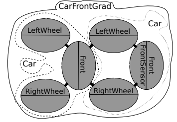
Fig. 2. Gradient field in RoCoRo applied to a configuration of two docked cars using concrete instantiations CarFrontGrad and FrontSensor which specialize (instantiate) GradiField and GradiSource respectively. The docked car configuration moreover contains two Car ensembles which each consists of three modules playing car-specific roles.
