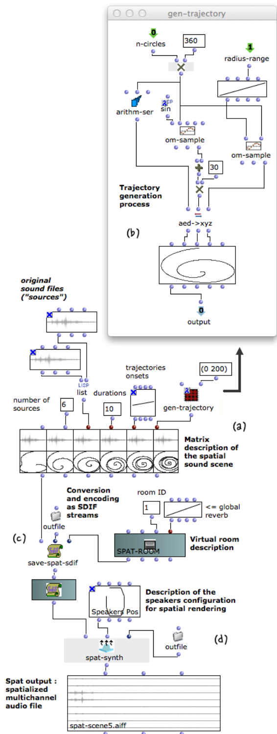
Fig. 1. Representation and rendering of a spatial sound scene in OpenMusic. The matrix representation of the scene (a) is instantiated from a set of sound sources and spatialization parameters provided either “literally” (e.g. durations, onsets...) or as functional specification (e.g. the trajectory generation process (b) provided as higher-order function). It is eventually encoded as an SDIF file (c), and here rendered to a multi-channel audio file (d).
