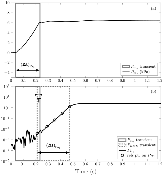
Figure 16: Example of the time evolution P_{H_1}(t) and P_{RMS}(t) for each value of (\Delta t)_{P_m} . A logarithmic scale is used for the ordinate axis.
