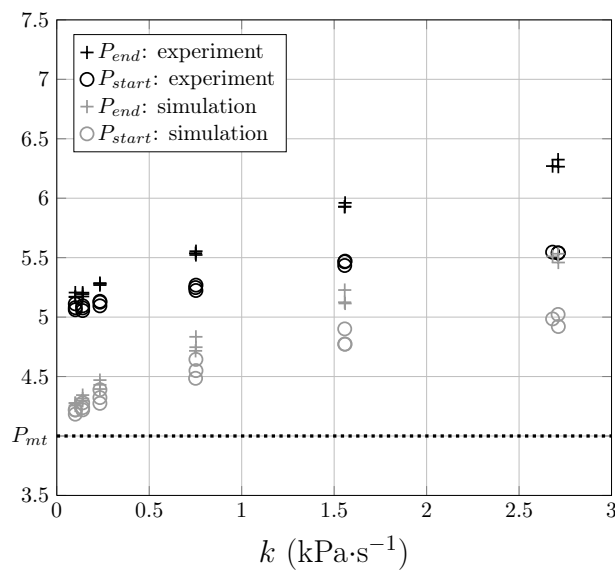
Figure 12: Graphical representation of P_{start} (o) and P_{end} (+) as a function of the slope k . The black marks are related to values obtained experimentally and the gray marks are related to values obtained on numerical simulation of Raman model.
