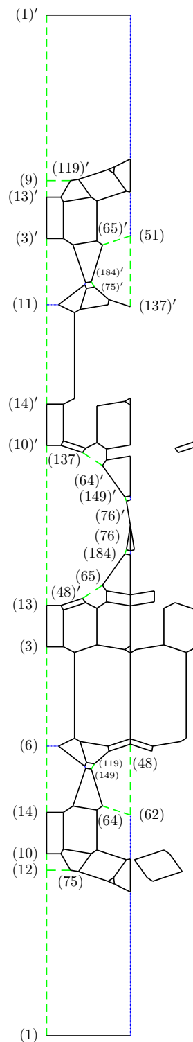
FIGURE 1. Fundamental domain in the case m = 37 .
