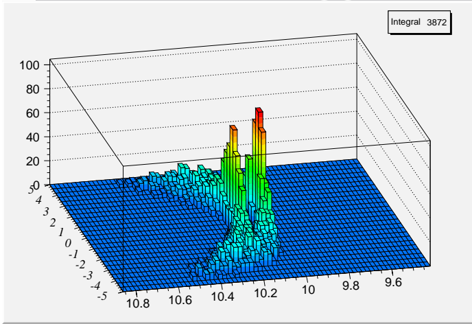
Figure 8: Example of the superposition on the focal plane of two Cherenkov patterns generated via Monte Carlo by one {}^9\text{Be} and one {}^{10}\text{Be} tracks both with a total particle momentum of 25 GeV/c.
