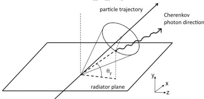
Figure 1: Definition of the \theta_y angle between the Cherenkov photon direction and the radiator plane. This angle is conserved during the light propagation along the bar and will be used throughout the paper as the measured quantity. For tracks at normal incidence, the Cherenkov half cone angle is the complementary angle: \pi/2 - \theta_y .
