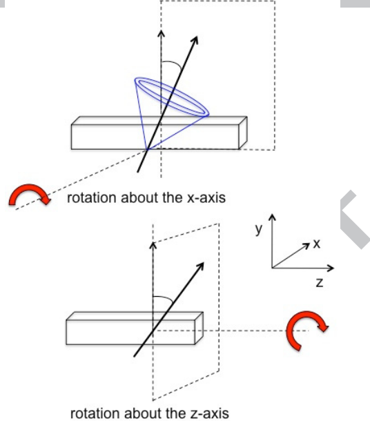
Figure 9: Definition of the tilt angles of the incident track with respect to the bar axes.
