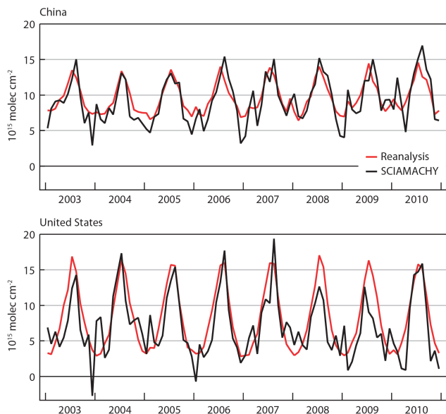
Fig. 31. Time series of monthly mean area-averaged tropospheric HCHO columns in 10^{15} molecules \text{cm}^{-2} from the MACC reanalysis (red) and IUP-SCIAMACHY (black) for China (top) and the eastern US (bottom). Only land points were used in these calculations.
