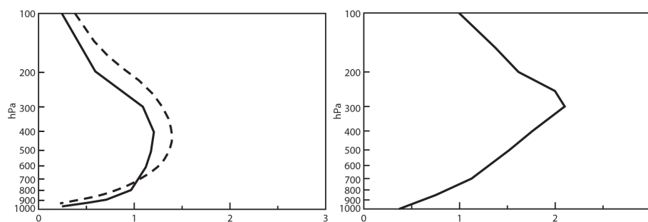
Fig. 1. Left panel: mean averaging kernels for MOPITT (solid) and IASI (dashed) daytime total column CO retrievals for July 2009 averaged over a 5^\circ \times 25^\circ box over Europe ( 46\text{--}51^\circ N, 3\text{--}28^\circ E). Right panel: global mean averaging kernels for tropospheric column \text{NO}_2 from SCIAMACHY averaged over the period June 2009 to May 2010.
