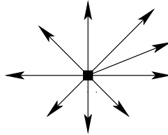
FIGURE 3.1. Repulsive point
