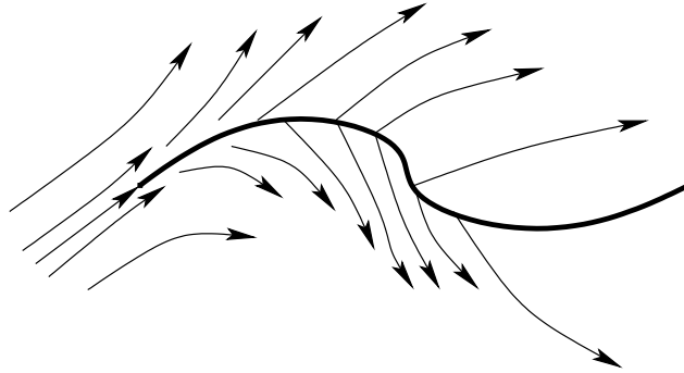
FIGURE 3.4. Incoming cutedge
