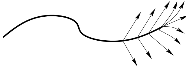
FIGURE 3.5. Outgoing cutedge
