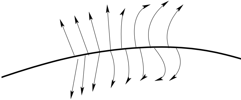
FIGURE 3.2. Around \mathcal{E}_\delta(V)
