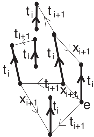
FIGURE 3. Other edges in E_i
