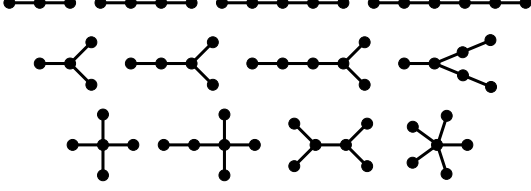
Figure 2. Our set \mathbb{T} of 12 tree patterns.
