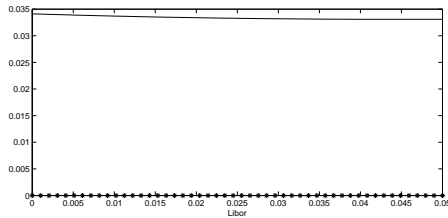
FIG. 4.7. The optimal boundary: \Gamma_1^* in regime X = e_1 (solid line) and \Gamma_2^* in regime X = e_2 (asterisk line) as function of the LIBOR r (x axis) and the intensity \lambda (y-axis) for the inputs in Section 4.2. Recall that the continuation region is above the boundary and the exercise region below the boundary. For regime e_1 two regions appear : the continuation region and the exercise region while for regime e_2 only the continuation region is present. The borrower will only prepay in regime e_1 after the crisis is over.
