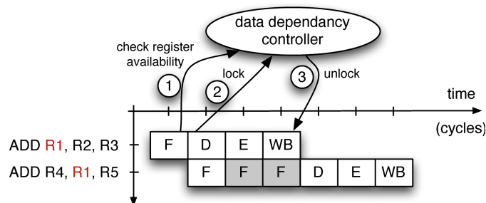
Figure 8: Interaction between the Data Dependency Controller and the pipeline model.
