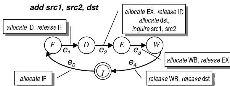
Figure 2: Madl OSM model example of the ADD instruction ( Qin et al. (2004) ).
