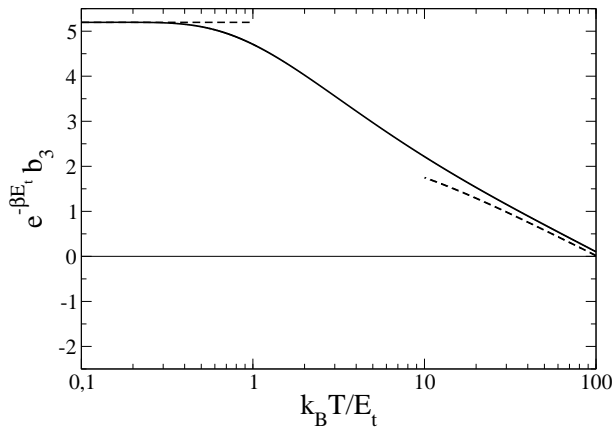
FIG. 1: Third cumulant b_3 of the spatially homogeneous unitary Bose gas: b_3 is multiplied by e^{-\beta E_t} and plotted as a function of temperature T as a solid line. The dashed lines to the left and to the right respectively correspond to the approximations (54) and (55), that have been multiplied by e^{-\beta E_t} . ( -E_t ) is the energy of the ground state (efimovian) trimer, and \beta = 1/(k_B T) .
