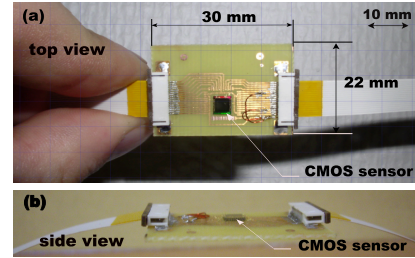
Fig. 3. Photography showing the final connection of the developed CMOS camera and integrated in the PCB support.
