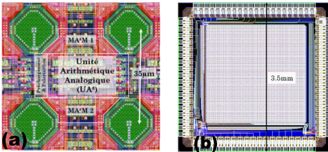
Fig. 2. (a) layout of 4 pixels and (b), full layout of the retina (64x64 pixels).
