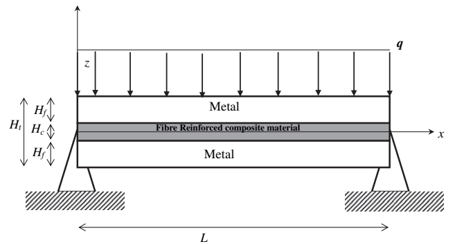
Fig. 1. Laminate beam with fibre Reinforced composite material core.
