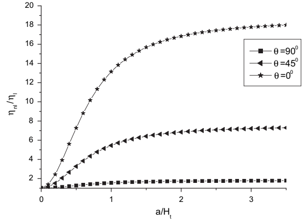
Fig. 3. Loss factor ratio \eta_{nl}/\eta_l as a function of the vibration amplitude ( a/H_t ) for various values of \theta with Touratier model; b = 1 ; H_f/H_c = 7 ; L/H_t = 100 .
