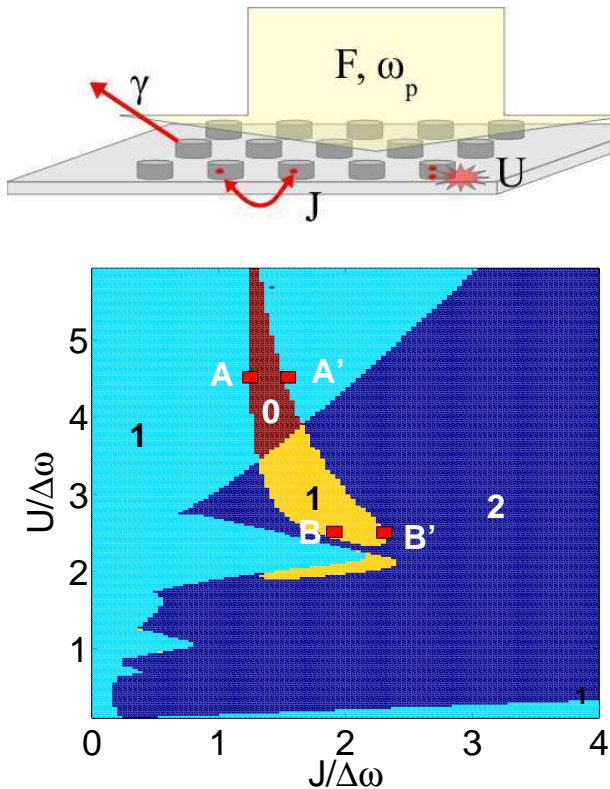
FIG. 1: Color online. Top: Sketch of a square photonic lattice made of nonlinear cavities coupled by tunneling. The system is pumped coherently by an homogeneous laser field at normal incidence. Bottom: Number of mean-field solutions plotted as a function of J/\Delta\omega and U/\Delta\omega , for F/\Delta\omega = 0.4 ; \gamma/\Delta\omega = 0.2 and \Delta\omega > 0 . Light blue (top-left and bottom-right part labeled with a ‘1’): monostable region, only one solution to Eq.(4). Dark blue part (label ‘2’): bistable region, two solutions to Eq.(4). Yellow part (central region labeled with ‘1’): has only one stable phase out of two existing solutions. Red part (label ‘0’): only one solution, which is unstable.
