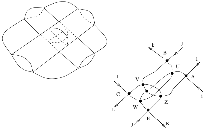
FIGURE 19. Kashaev's configuration at crossings.
