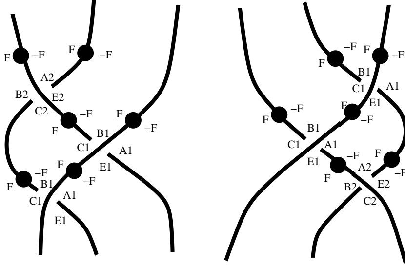
FIGURE 12. Braid Reidemeister move III.
