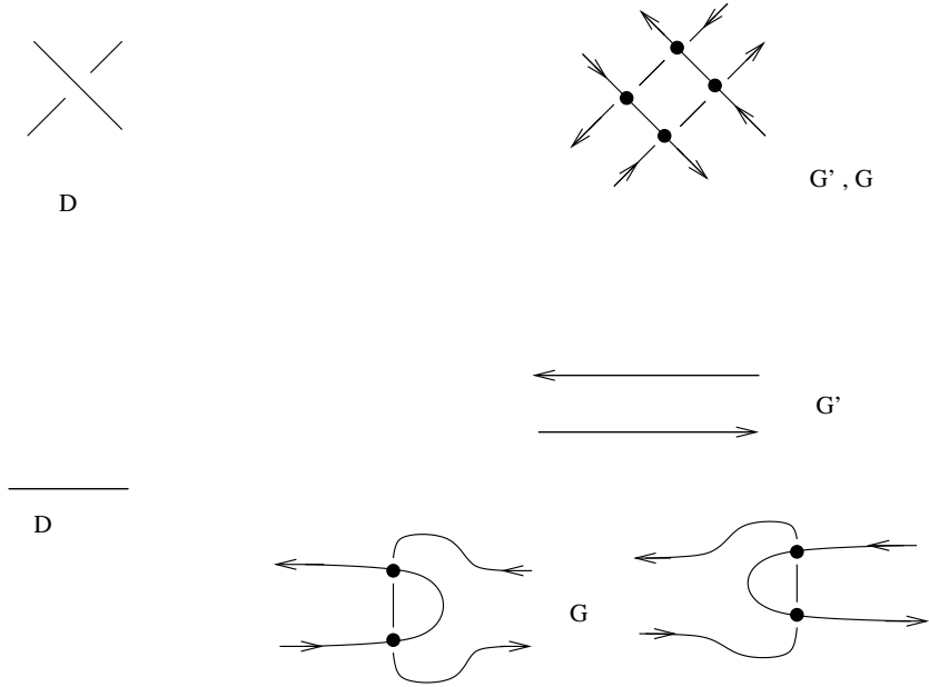
FIGURE 5. From link diagrams to o-graphs.
