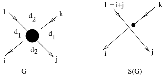
FIGURE 4. Matrix dilogarithm \mathcal{R}_N(-, d)_{i,j}^{k,l} and S-graph: *_b = -1 .
