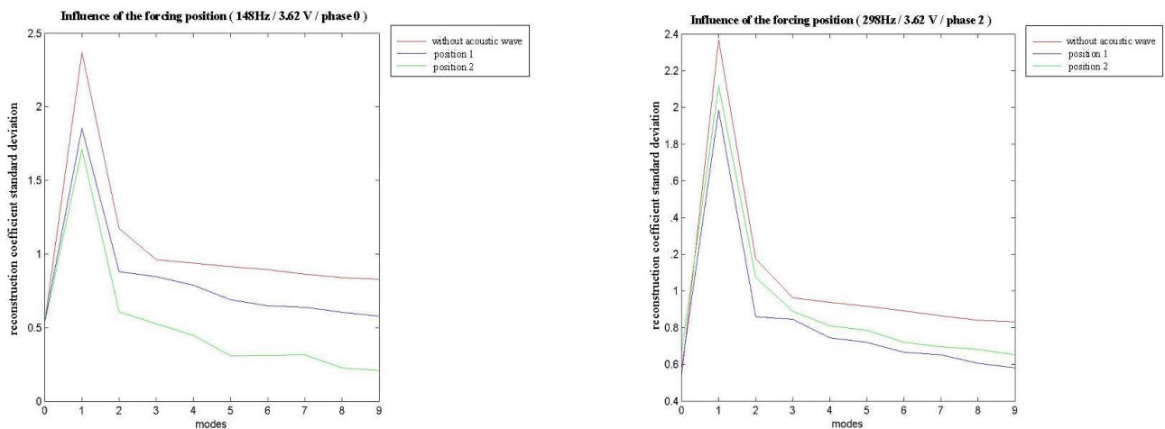
Fig. 12 P.O.D. results of square reconstruction coefficients for all modes : (a) forcing acoustic wave with a frequency equal to 150Hz (natural frequency), (b) forcing acoustic wave with a frequency equal to 300Hz (double harmonic frequency).
