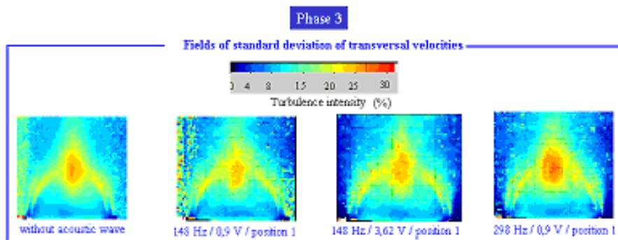
Fig. 9 Influence of the amplitude and the frequency of the acoustic wave (Reynolds decomposition radial and longitudinal fluctuations for the phase 3).
