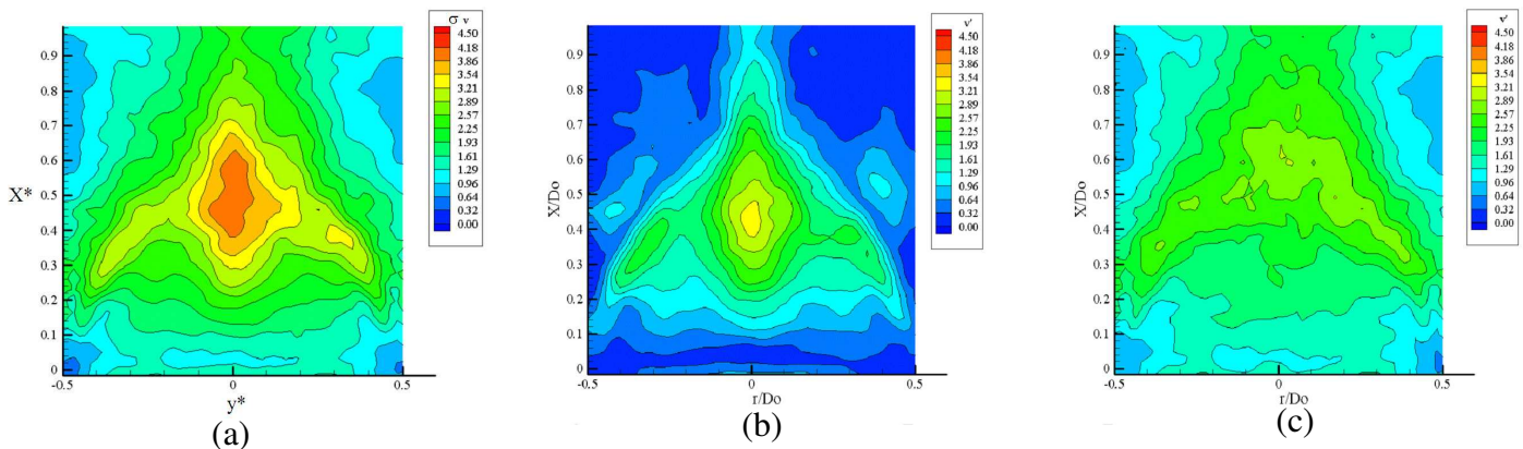
Fig. 6 Effect of the mode 1 on Reynolds decomposition radial velocity fluctuations: (a) Radial velocity fluctuations calculated with all velocity fields, (b) Radial velocity fluctuations reconstructed with mode 0 and 1, (c) Radial velocity fluctuations reconstructed without mode 1.
