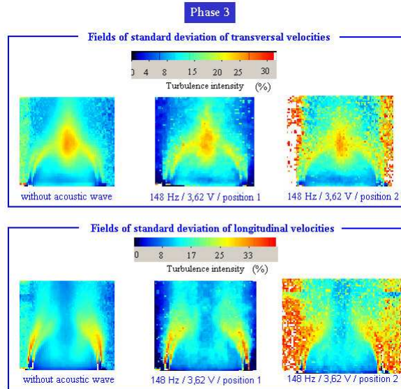
Fig.11 Influence of the loudspeaker position (Reynolds decomposition of radial and longitudinal fluctuations for the phase 3).
