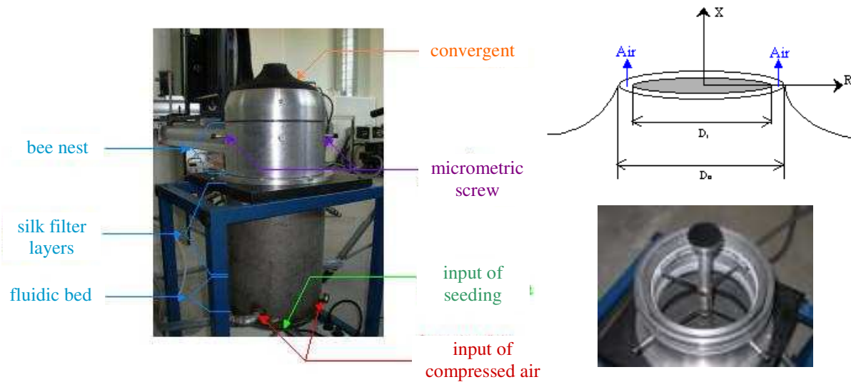
Fig. 2 Structure of the annular jet nozzle
