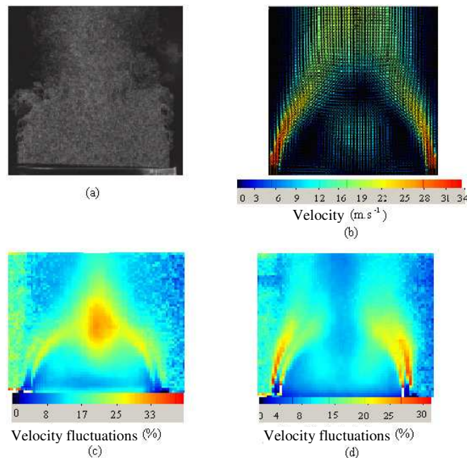
Fig.4 P.I.V. results for a natural annular jet flow (calculated with 1000 instantaneous fields): (a) instantaneous flow image, (b) average velocity field ( ReD_0=107\ 760 ), (c) radial velocity fluctuations, (d) longitudinal velocity fluctuations.
