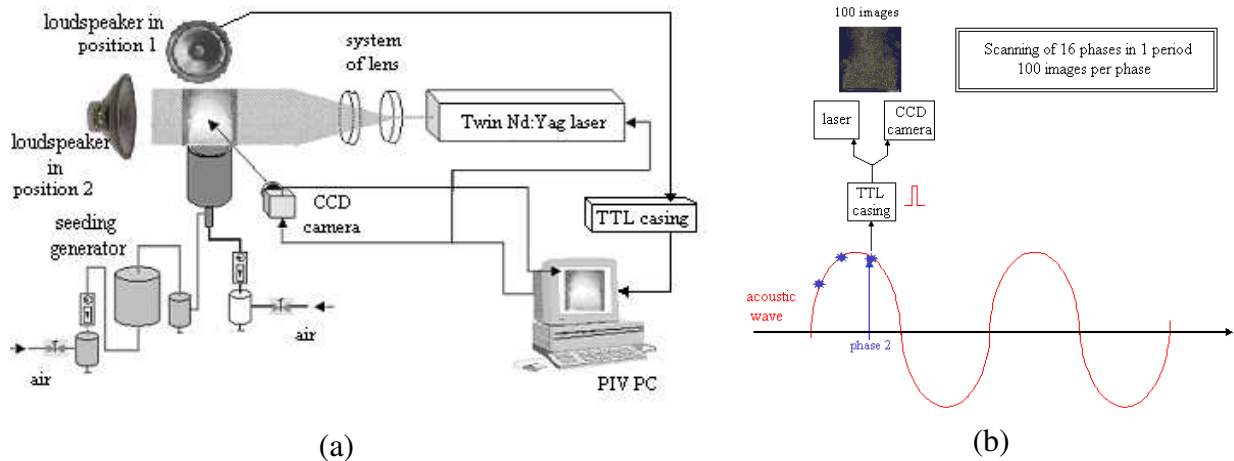
Fig. 3 (a) Diagram of the phased set-up used for the study of acoustic forcing, (b) Principle of the phased P.I.V. acquisition set-up.
