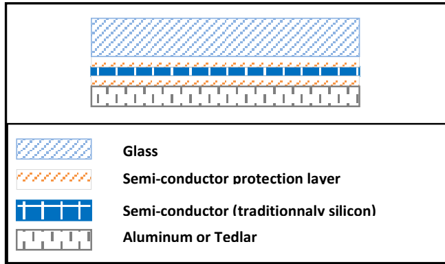
Fig 3. Cross section of a typical photovoltaic panel
