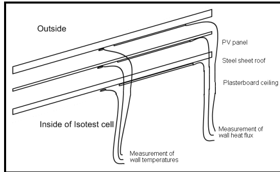
Fig 10. Sensors installation in the roof wall.
