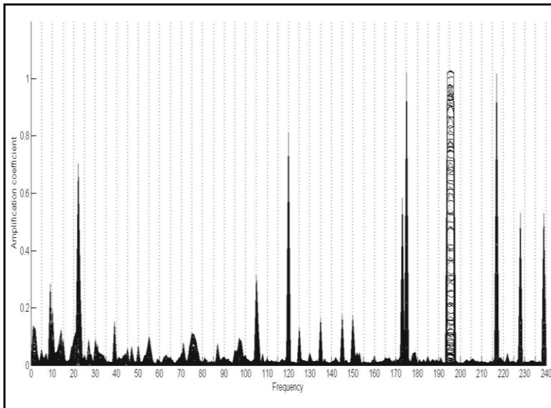
Fig. 13. Fourier spectrum of the sensitivity analysis for the inside air temperature of the building
