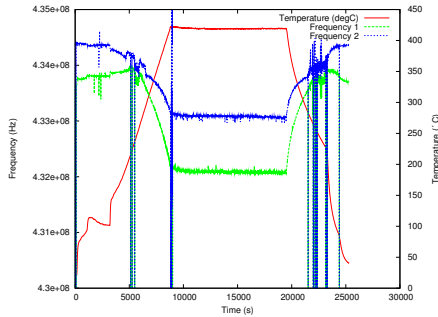
Figure 5. Behavior of resonator at intermediate temperature (around 450°C).
