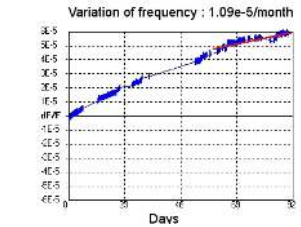
Figure 11. Variation of frequency of the oscillator over time ( 1.09 \times 10^{-5} for LGS versus 10^{-7} )
