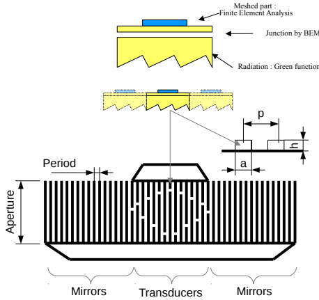
Figure 1. FEM/BEM synoptic.
