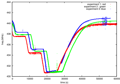
Figure 13. Behavior of a langasite sensor. The experiment cycle is divided in 3 steps, 300 °C, 500 °C and 700 °C for 2h at each temperature.
