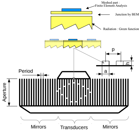
Figure 1. FEM/BEM synoptic.
