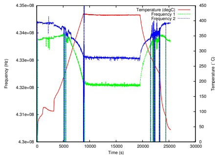
Figure 5. Behavior of resonator at intermediate temperature (around 450°C).
