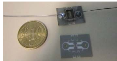
Figure 3. The different stages of the packaging process.
