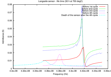
Figure 12. Life time test: temperature cycles are performed from room temperature to 700°C during 10h, showing a life time of 30 hours.
