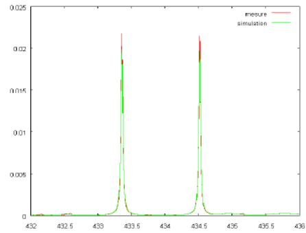
Figure 2. Comparison between computation and measurement of the TSEAS10 double resonators sensor.
