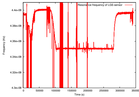
Figure 8. Wireless measurement of the sensor at 500°C during 50h. Between 0s and 50000s, the sensor is packaged (Fig3) and placed in the oven for a first preliminary cycle (100°C for 2h, 270°C for 2h and 360°C for 2h). Between 80000s and 280000s, the sensor withstands a temperature of 500°C.
