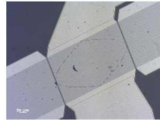
Figure 6. Picture of the IDT of TSEAS10 sensor used during 50 hours at 450°C while measured by wireless interrogator. IDT are polluted after the opening of the ceramic package using milling tools.
