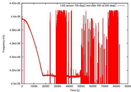
Figure 9. Wireless measurement of the sensor at 700°C. Between 0s and 18000s, the oven is warming up. The sensor is then operating at 700°C during 36000s (from 18000s to 54000s), then the sensor does not operate anymore.
