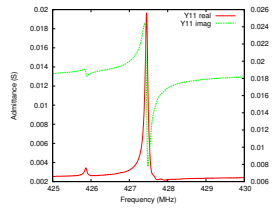
Figure 10. Reponse of the resonator used in the oscillator loop.
