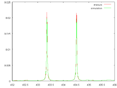
Figure 2. Comparison between computation and measurement of the TSEAS10 double resonators sensor.
