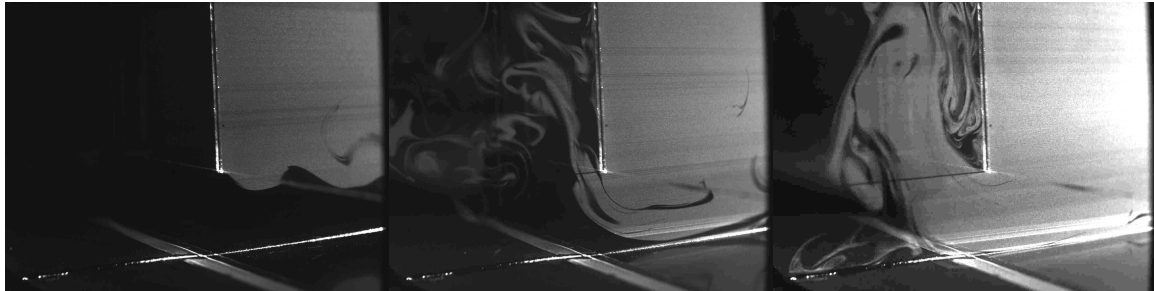
(a) H_s=37\text{mm} ( Fr=1,29 ) (b) H_s=27\text{mm} ( Fr=2,16 ) (c) H_s=17\text{mm} ( Fr=4,71 )
