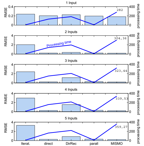
Fig. 9. RMSE versus computing time for various number of inputs.
