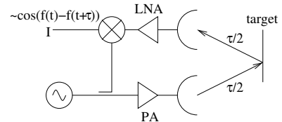
Figure 1. In case of a static target, a CW RADAR receiver noise detection limit is associated with the local oscillator frequency fluctuation between the emitted pulse at time t and the received pulse delayed by \tau , the two-way transit duration.
