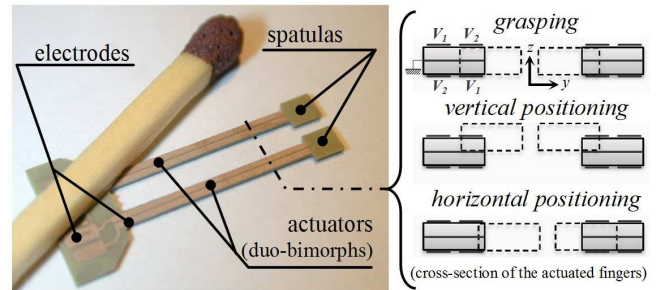
Fig. 2. Piezoelectric actuators on which the fingers (Fig. 1 (a)-(b)) are glued. Each finger is actuated by the piezoelectric actuator with four electrodes to enable four degrees of freedom of mobilities.
