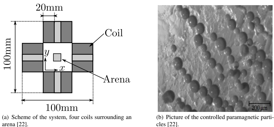
Fig. 10 Design of the paramagnetic particles controlling system.
