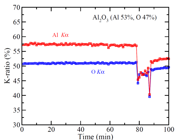
Figure 7. k -ratio for Al and O, as a function of irradiation time, measured on a \text{Al}_2\text{O}_3 insulator sample. Beam energy and beam current are 2.5 keV and 500 nA, respectively.
