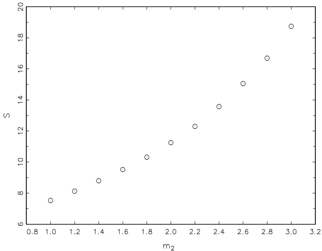
Figure 8: Values of S matching moments ( m_1 = 6 and m_2 \in [1;3] ) - Minimum
