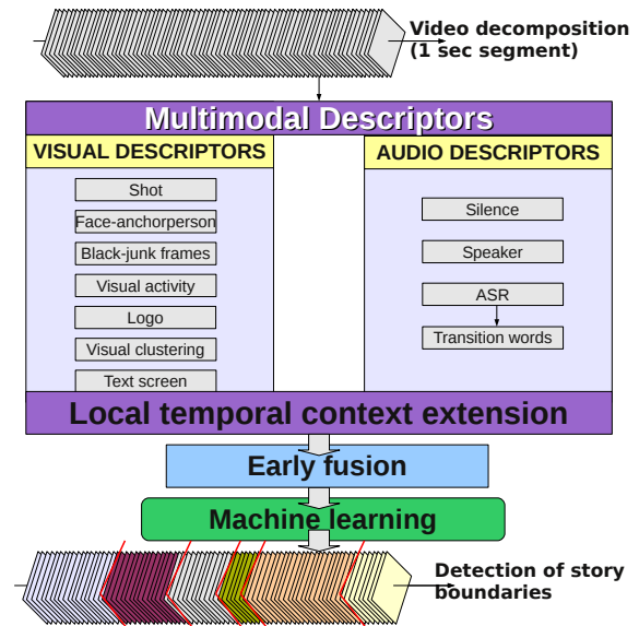
Figure 1. Multiple Descriptors Based Story Segmentation
