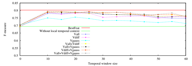
Figure 5. Results for local temporal context
