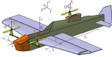
Fig. 2. Vertical flight (helicopter mode)
