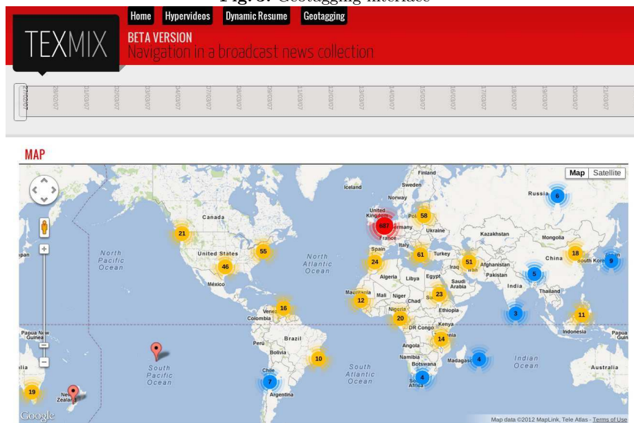
Fig. 3. Geotagging interface
