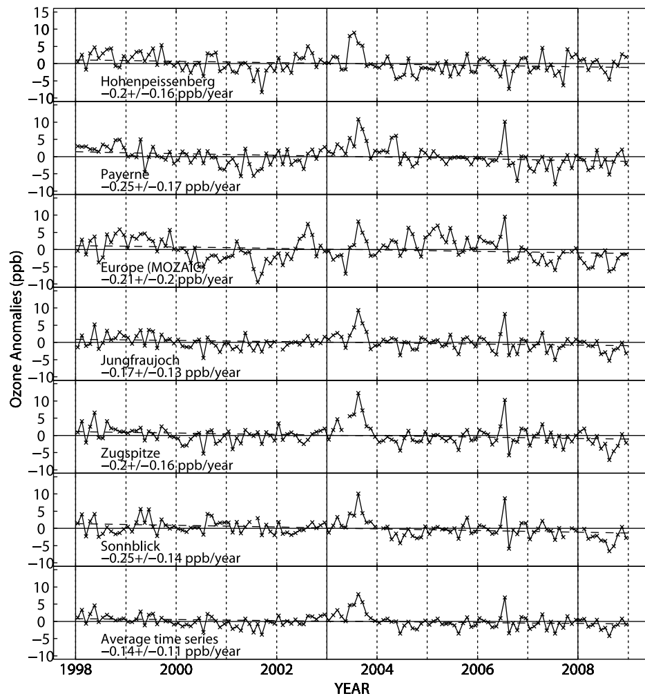
Figure 12. Annual trends in ozone ( \text{ppb yr}^{-1} ) for the alpine sites and for Hohenpeissenberg, Payerne, and the MOZAIC mean time series at 681 hPa (2.6–3.8 km), and for a time series composed of the average of the monthly mean time series for these six locations (bottom panel). The annual trends are superimposed on monthly anomalies computed relative to monthly means for 1998–2008. The trend regression model is described in the text, equation (1). Two standard errors are shown.
