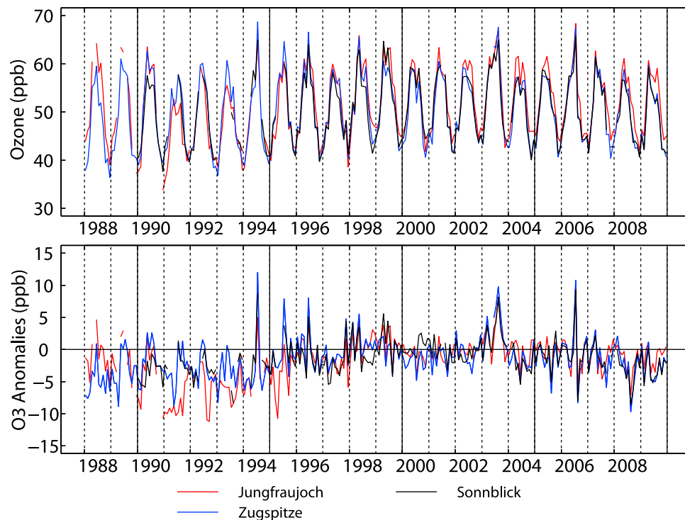
Figure 5. (top) Monthly mean time series for ozone (in ppb) at the alpine sites. (bottom) Monthly anomalies (in ppb) relative to the monthly means for January 1997 to December 2003.
