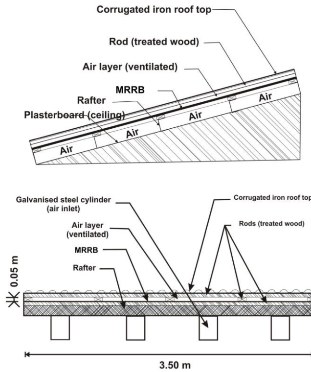
Figure 4: Section and front view of the specific roof installed for the study of MRRB (Multi-Reflective Radiant Barriers)
