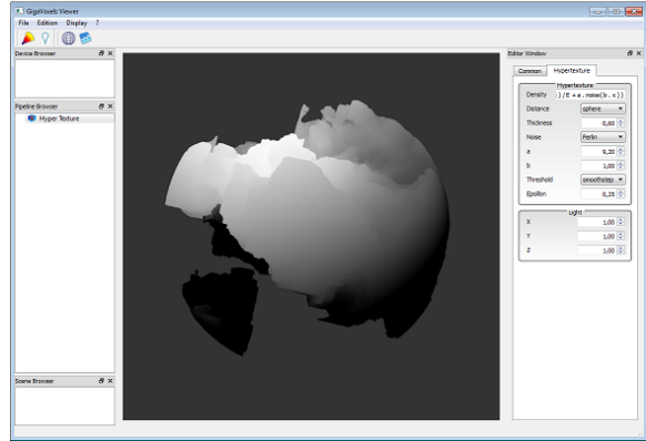
Figure 17: Viewer GigaVoxels
