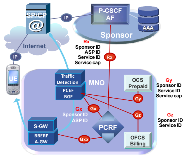
Figure 3: Sponsor intermediary between MNO and ASP
