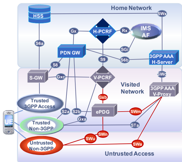
Figure 1: Untrusted Access in Roaming
