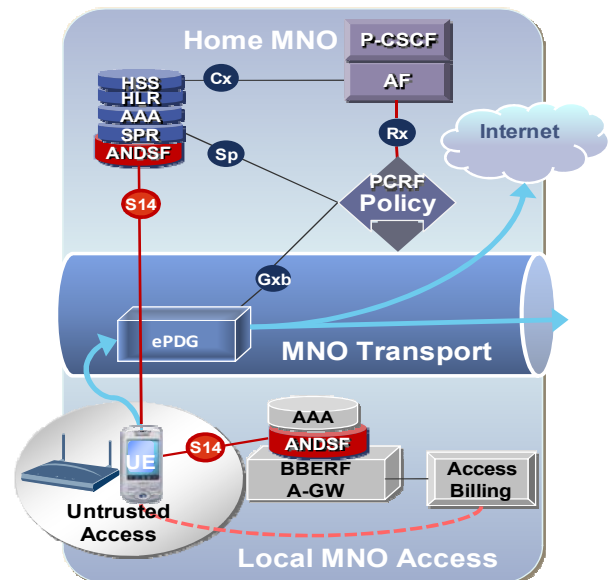
Figure 2: Untrusted Access Admission
